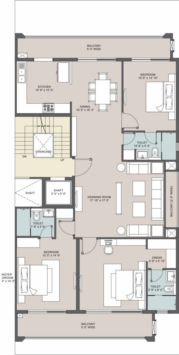
Typical Floor
