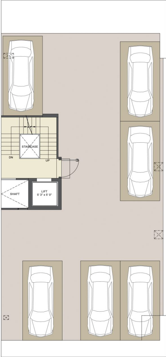
Stilt Floor
